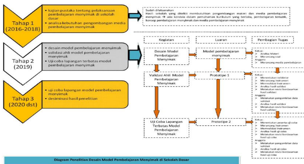
Diagram 2.1 Alur Penelitian
